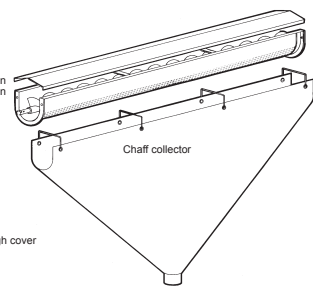
8 foot screen cleaning section
