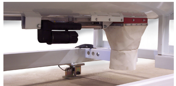
Optional electric gate discharge
